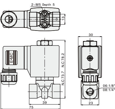
ELP06/08 Direct Acting Type
