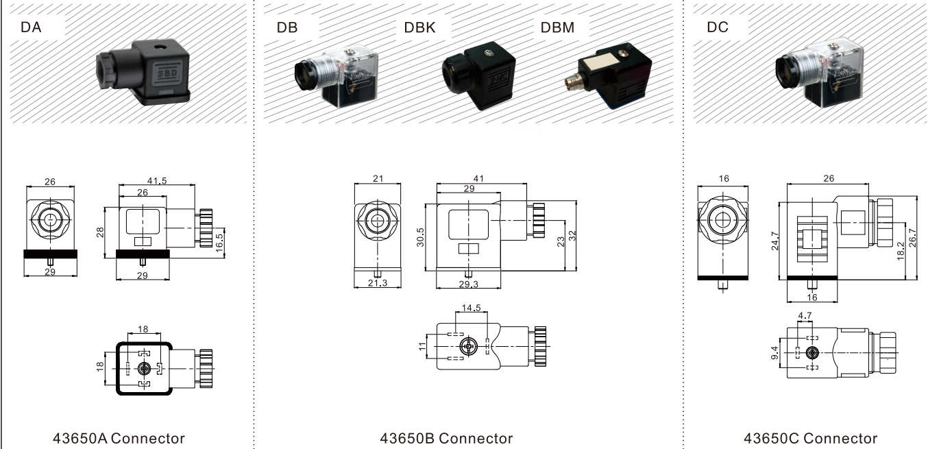
43650A Connector
