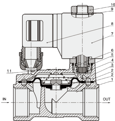
Pilot Type
