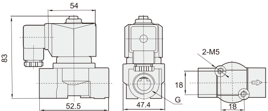
Φ4mm 3/8"
